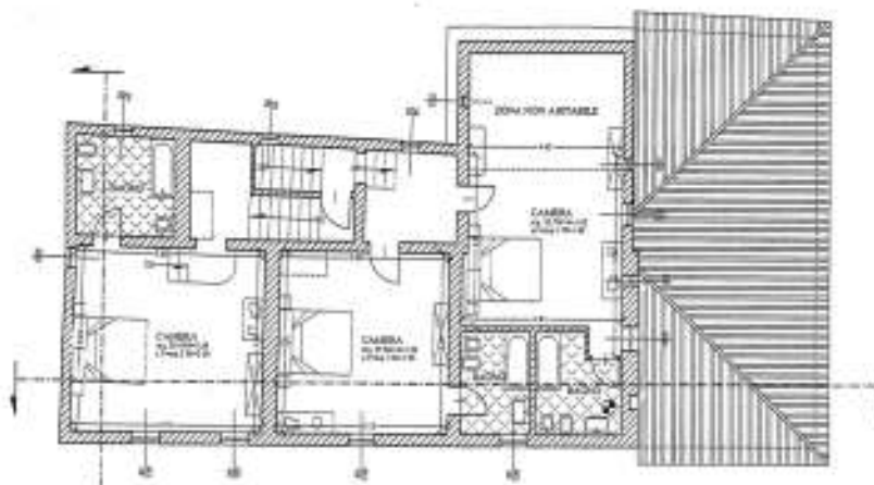
SECONDO PIANO / SECOND FLOOR
