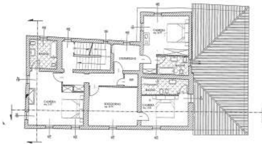
PRIMO PIANO / FIRST FLOOR
